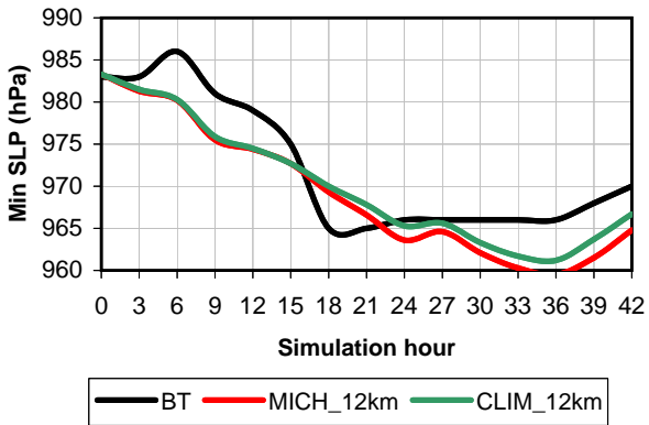
Min SLP - Hurricane Michael (12km)
