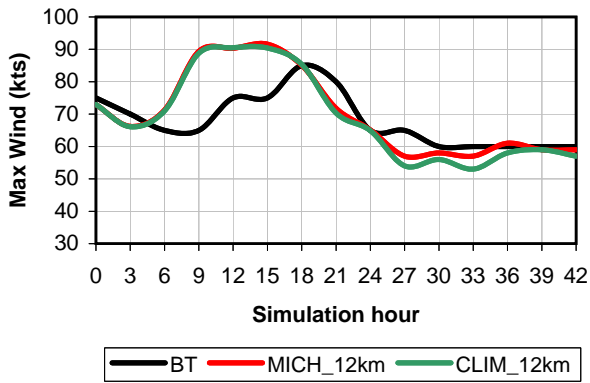
Max Wind - Hurricane Michael (12km)
