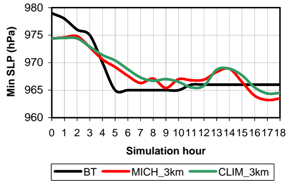
Min SLP - Hurricane Michael (3km)
