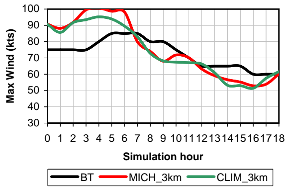
Max Wind - Hurricane Michael (3km)
